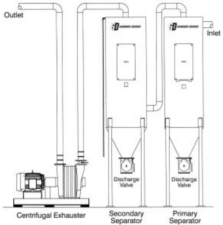
MULTISTAGE CENTRIFUGAL EXHAUSTER SECONDARY COLLECTOR PRIMARY COLLECTOR
